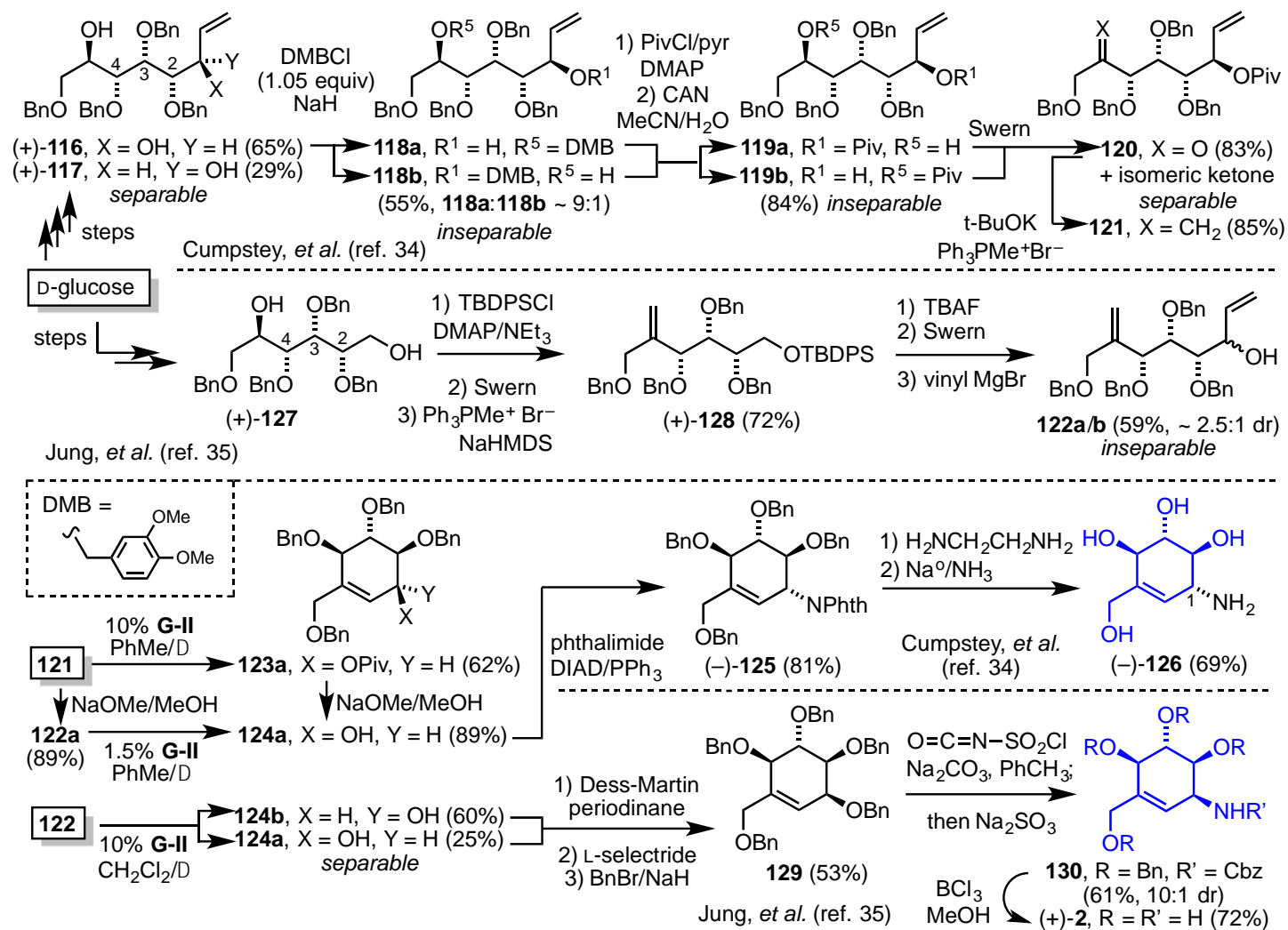
Scheme 17. Synthesis of \beta -valienamine 126 and valienamine 2 via RCM from D-glucose.
