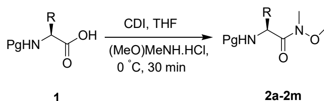
Scheme 1. Synthesis of N^\alpha -protected Weinreb amides.
