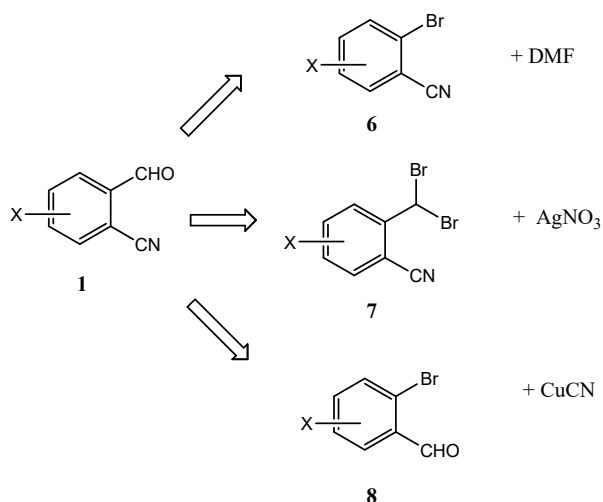
Figure 2. Common approaches to 2-formylbenzonitriles.
