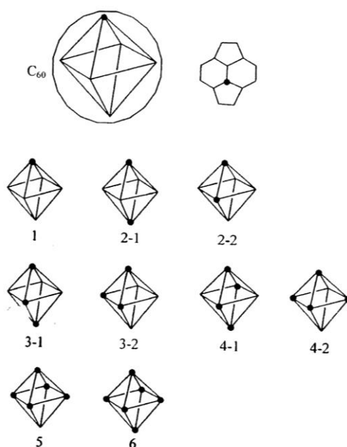
Figure 1. Regioselective scheme of addition of the same addends to C_{60} . 11
