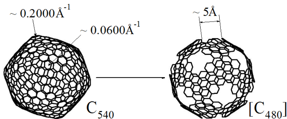
Figure 11. Carbon cages of C_{540} fullerene and a possible product of ozone annealing of the regions of the C_{540} surface with the highest curvature. 40
