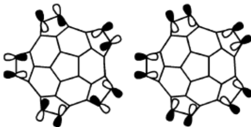
Figure 6. Schematic representation of HOMO ( left ) and LUMO ( right ) of C_{50} ( D_{5h} ). 33
