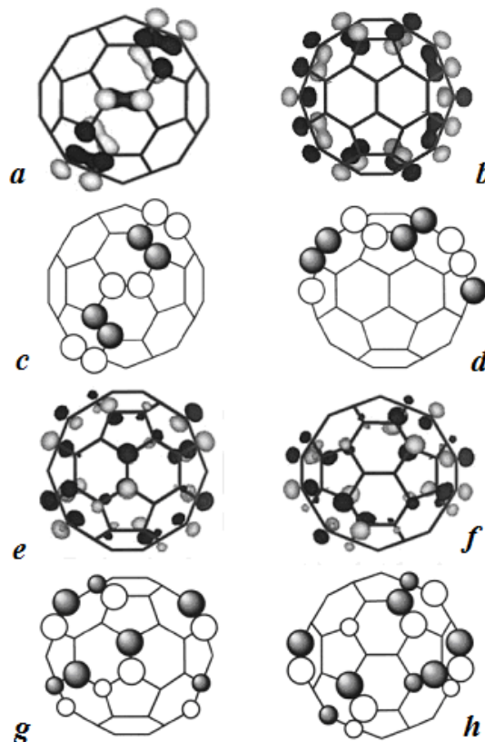
Figure 5. Frontier molecular orbitals of C_{60} (calculated by PM3 method): a, b – two projections of 5 degenerated HOMOs; c, d – respective projections of schematic representation of exohedral parts of HOMOs; e, f – two projections of 3 degenerated LUMOs; g, h – respective projections of schematic representation of exohedral parts of LUMOs. 29
