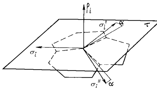
Figure 4. Orbitals of one of the carbon atoms in the C_{60} molecule. 26
