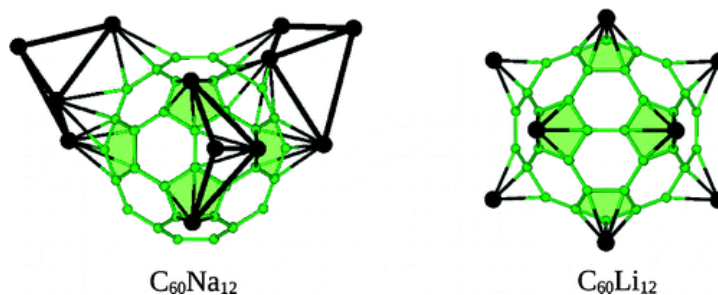
Figure 2. Equilibrium structures of alkali- C_{60} nanoclusters. 18
