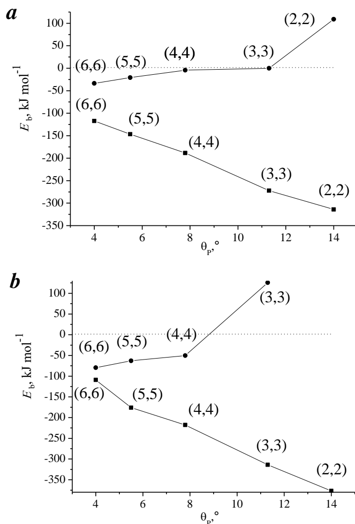
Figure 14. The dependence of exohedral (■) and endohedral (●) binding energies E_b calculated by B3LYP/6-31G* method on the pyramidal angles of (n,n) nanotubes ( n = 2-6 ): a – addition of H•, b – addition of F•. 48
