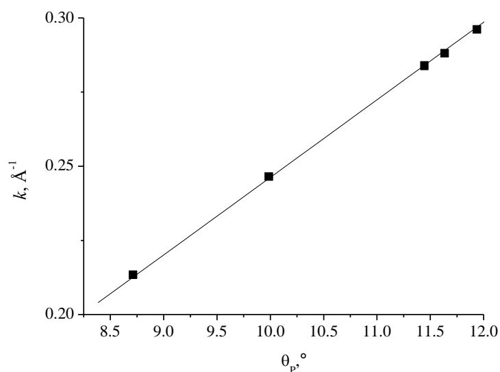
Figure 8. The correlation between pyramidity angles and carbon surface curvature. 39
