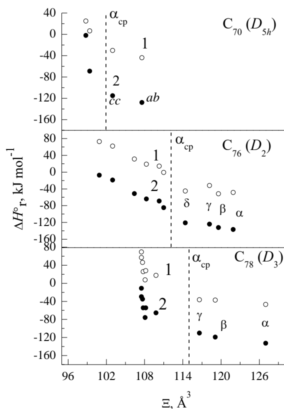
Figure 16. Heats \Delta H_r^\circ of addition of (1) diazomethane and (2) ozone to fullerenes ( \Delta H_r^\circ ) vs. polarizability indices of 6.6 bonds. 52
