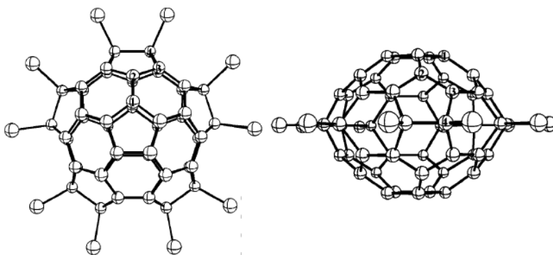
Figure 7. The structure of C_{50}Cl_{10} . 34
