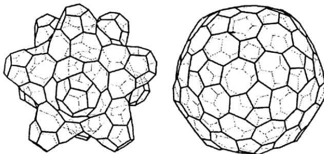
Figure 15. Hypothetical fullerene-like nanoclusters constructed with 72 pentagons (regions of positive curvature) and 60 heptagons (regions of negative curvature). 51
