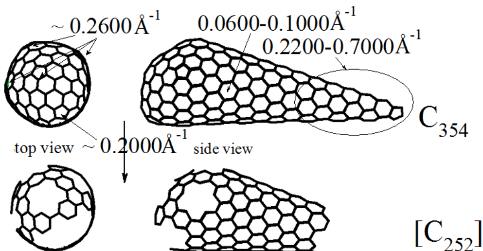
Figure 12. Carbon cages of C_{354} nanocone and a possible product of ozone annealing of the regions of the C_{354} surface with the highest curvature. 42
