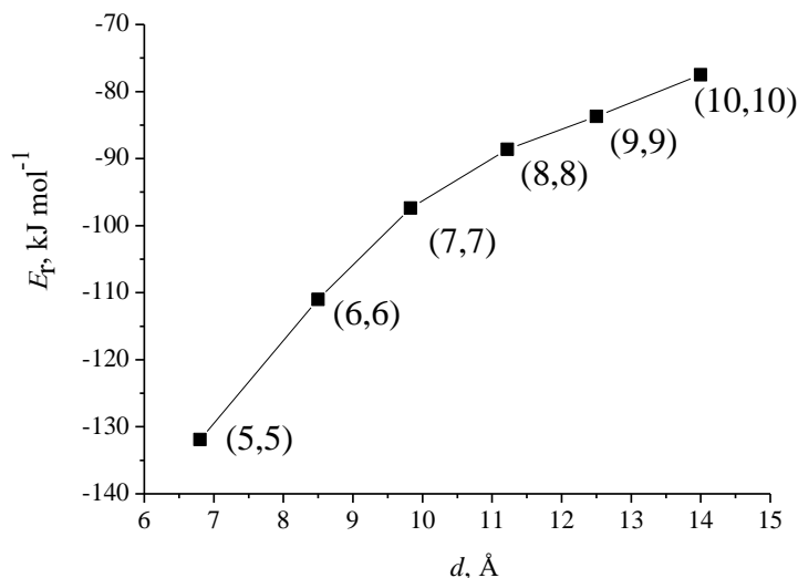
Figure 13. Exothermicity E_r of 1,3-dipolar addition of ozone to (n,n) nanotubes vs. their diameter. 44
