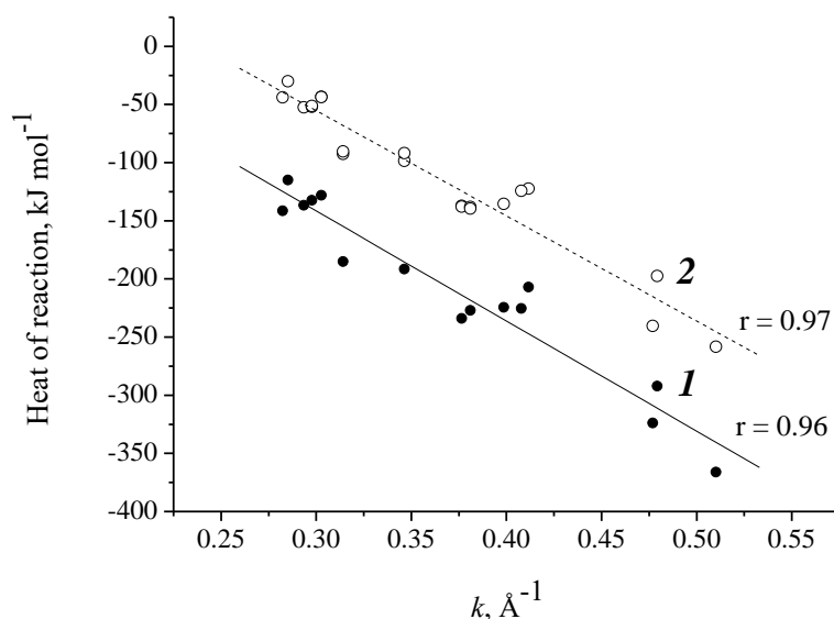
Figure 10. Correlations between heats of addition ( \Delta H_r^\circ ) of ozone ( 1 ) and diazomethane ( 2 ) to fullerenes and curvature indices. 40
