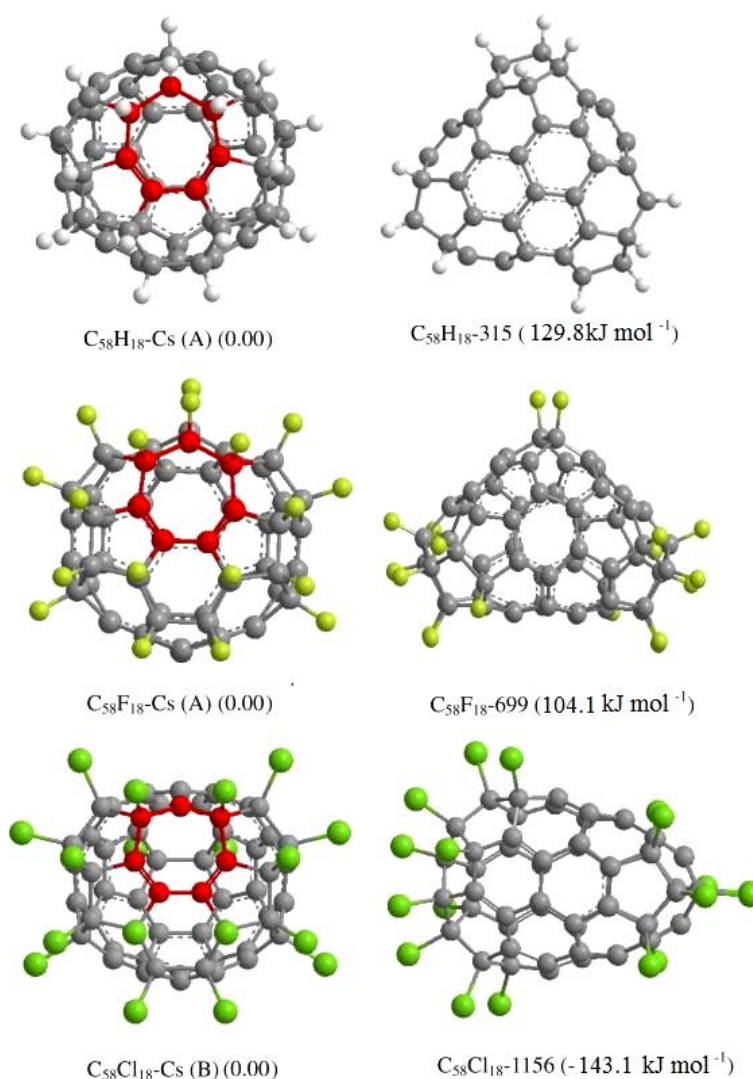
Figure 3. The optimized structures of the lowest-energy classical and non-classical fullerene derivatives C_{58}X_{18} ( X = H, F, Cl ) at the B3LYP/6-31G* level (relative energies are in the parentheses). 22
