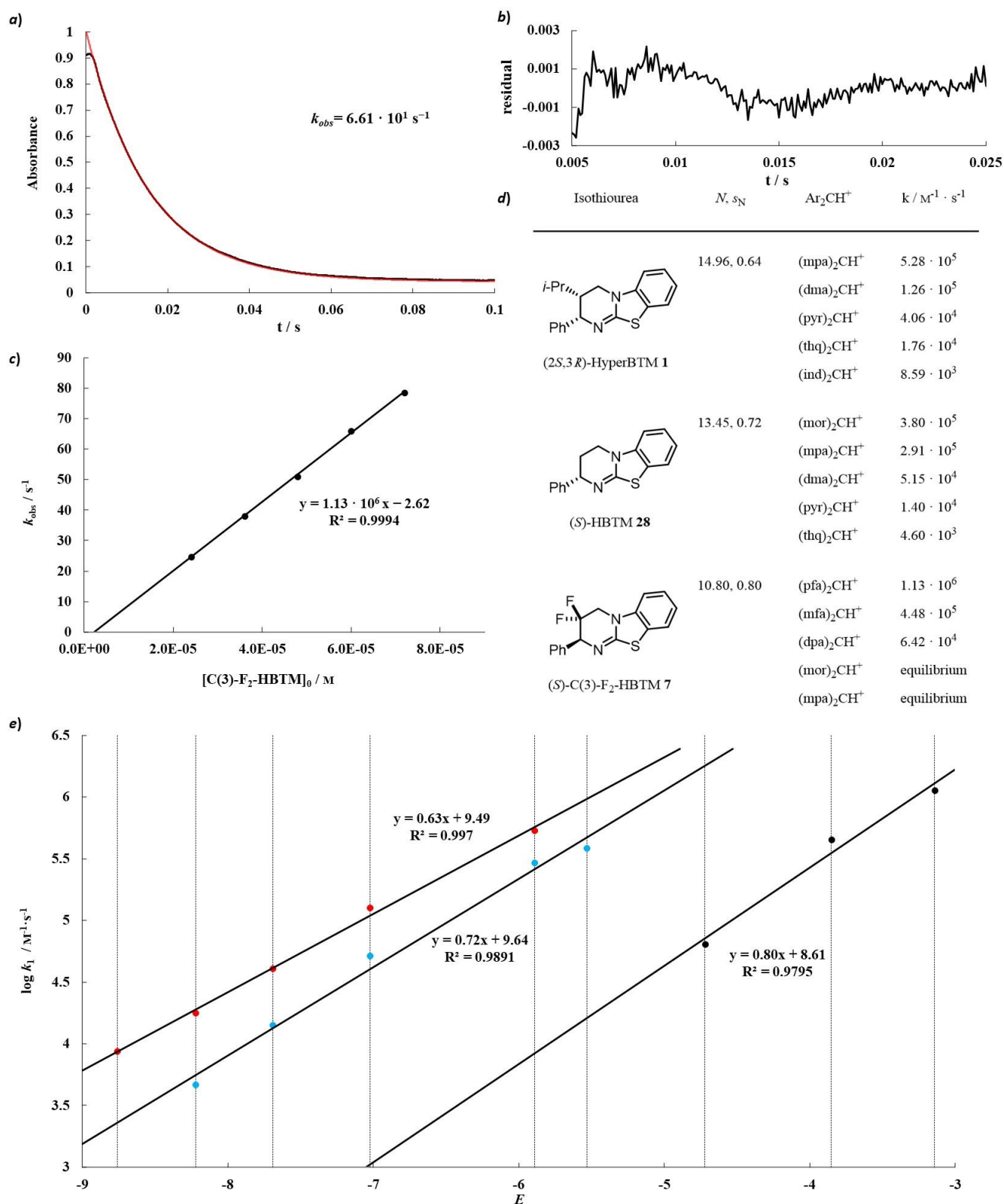
a) Absorbance at 601 nm during the reaction of 7 ( c = 6 \cdot 10^{-5} \text{ M} ) with (pfa) 2 CH + BF 4 - 37 ( c = 6 \cdot 10^{-6} \text{ M} ) at 20 °C in CH 2 Cl 2 as an average of 5 runs and exponential fit using ExpoFit programme; the concentration is the concentration in the mixing cell. b) Difference of observed and fitted absorbance in the fitted region. c) Determination of the second-order rate constant k_1 = 1.13 \cdot 10^6 \text{ M}^{-1} \cdot \text{s}^{-1} from the dependency of k_{obs} on the concentration of C(3)-F 2 -HBTM 7 . d) Plot of \log k_1 for the reactions of HyperBTM 1 (red), HBTM 28 (blue) and C(3)-F 2 -HBTM 7 (black) with benzhydrylium ions (in order from left to right: (ind) 2 CH + BF 4 - 29 , (thq) 2 CH + BF 4 - 30 ,
