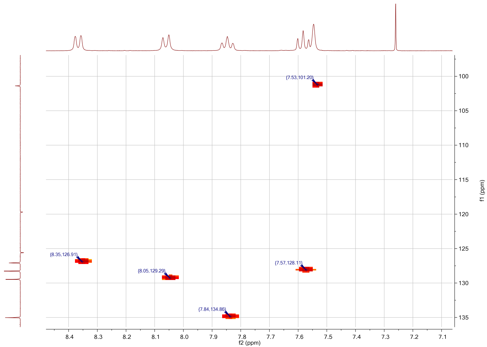
HSQC spectrum of 2,3-dimethyl-2 H -pyrazino[2,1- b ]quinoxaline-1,6-dione ( 3f ) (400 MHz, CDCl 3 )
