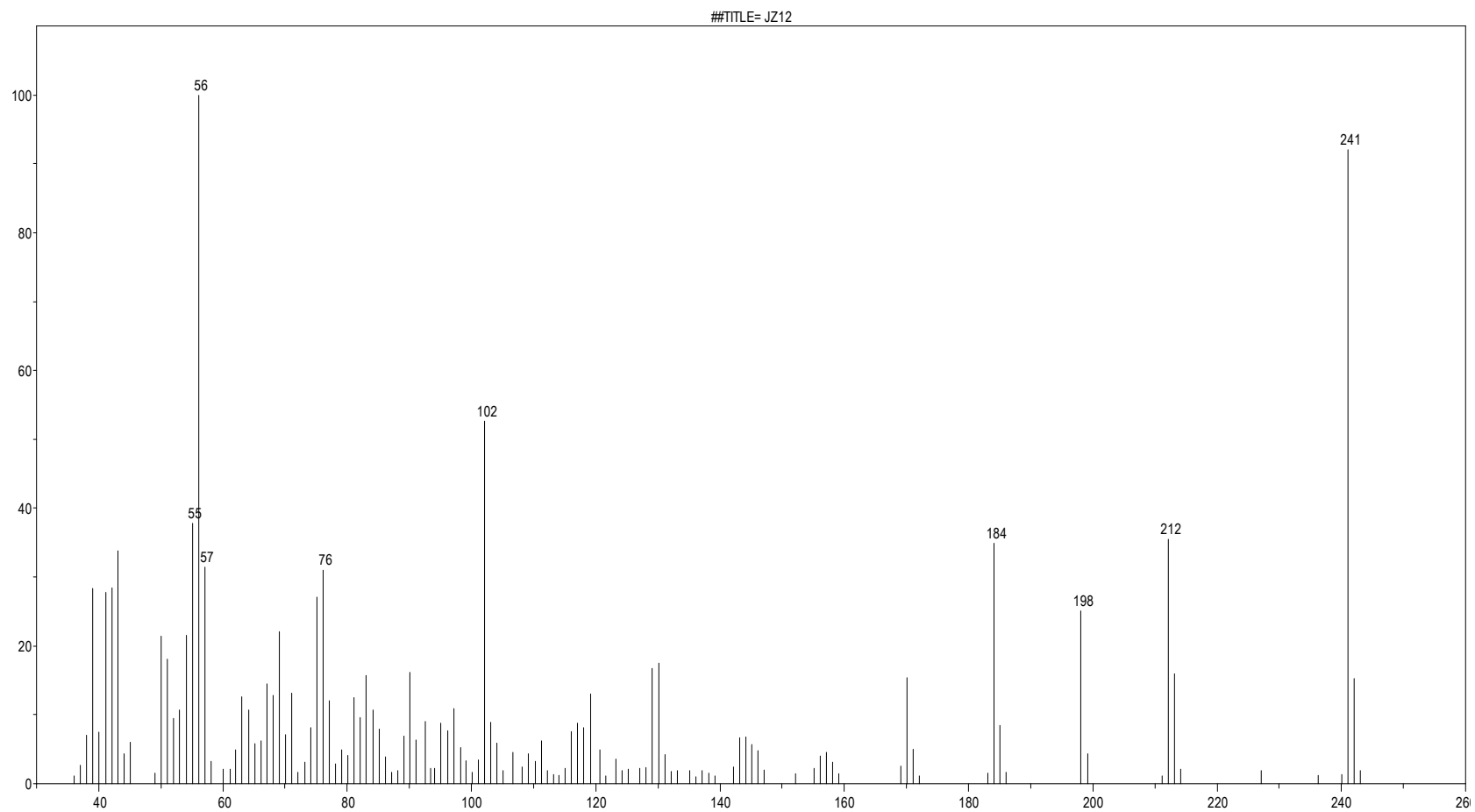
Mass spectrum of 2,3-dimethyl-2 H -pyrazino[2,1- b ]quiazoline-1,6-dione ( 3f )
