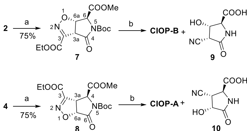
Scheme 3. Reagents and conditions: a: \text{RuO}_2 \cdot \text{H}_2\text{O} , \text{NaIO}_4 , \text{H}_2\text{O}/\text{AcOEt} ; b: \text{HCl} 6N, \Delta .
