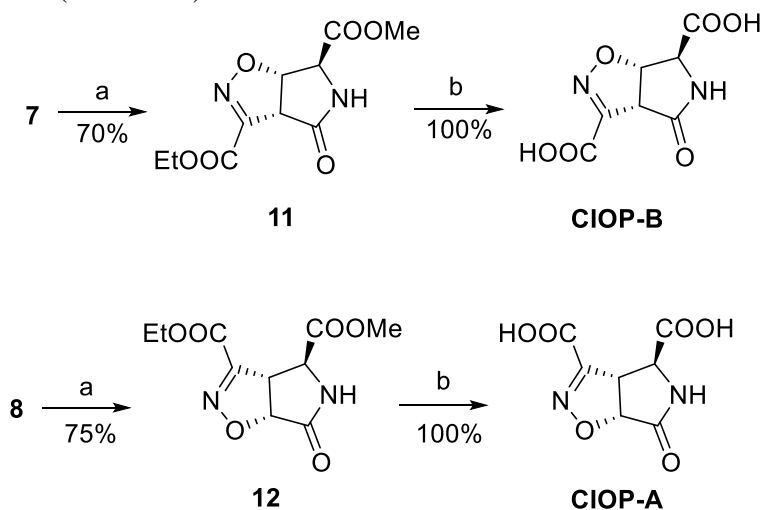
Scheme 4. Reagents and conditions: a: 30% TFA/ \text{CH}_2\text{Cl}_2 ; b: \text{K}_2\text{CO}_3 , \text{H}_2\text{O} .
