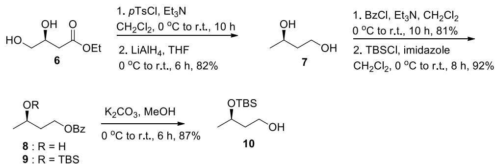
Scheme 2. Synthesis of compound 10 .
