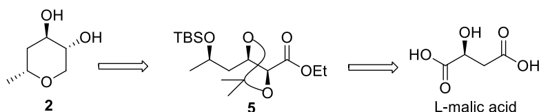
Scheme 1. Retrosynthetic route to the target molecule 2 .
