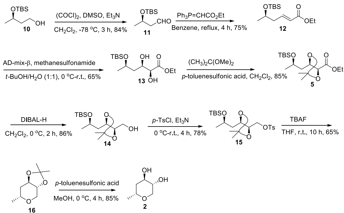
Scheme 3. Synthesis of target compound 2 .
