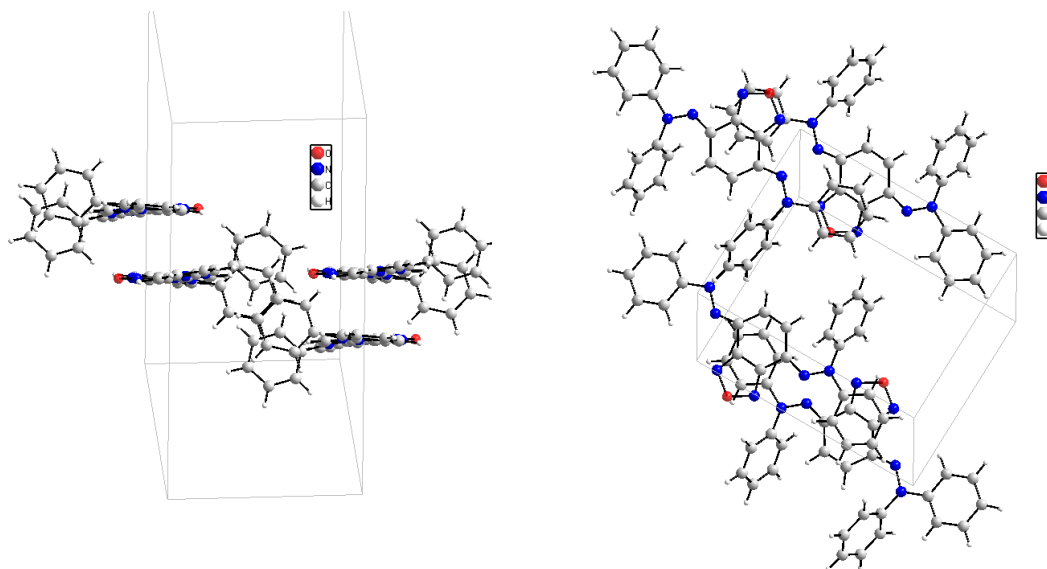
Figure S1. Crystal packing diagrams of 4 showing strong \pi - \pi interactions between the furazan moiety and an N-phenyl group.
