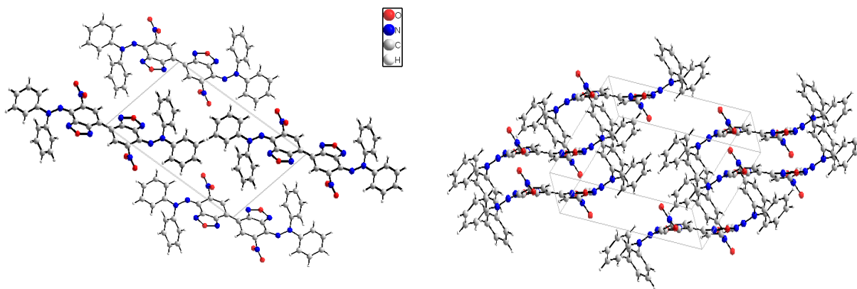
Figure S2. Packing diagrams of 13 in the crystal.
