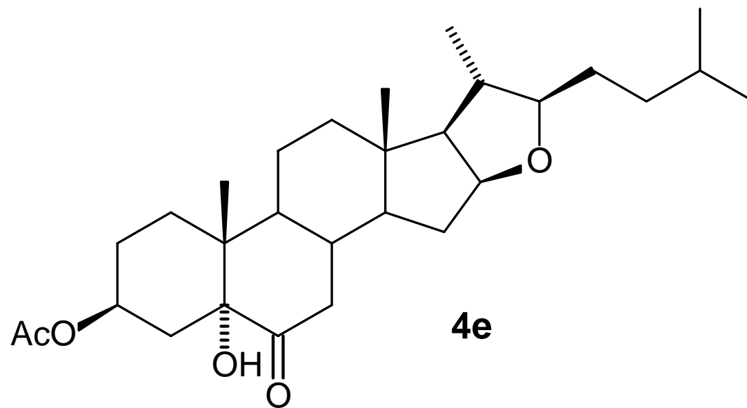
(22 R )-3β-acetoxy-5-hidroxy-5α-furostan-6-one
