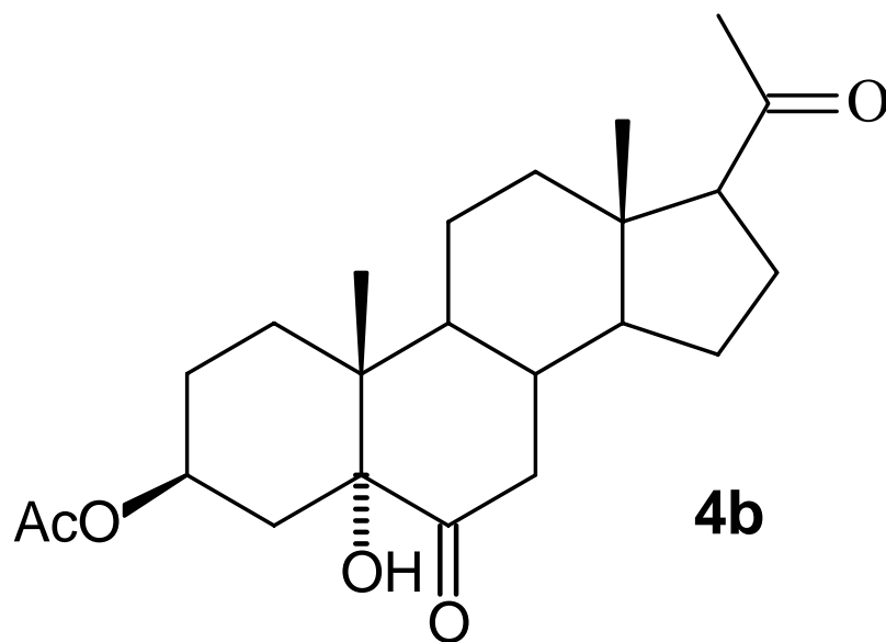
3β-acetoxy-5-hydroxy-5α-pregnan-6,20-dione
