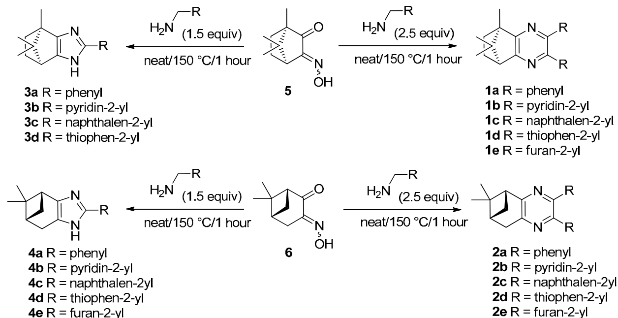
Scheme 1. Syntheses of pyrazines 1 and 2 as well as imidazoles 3 and 4 .
