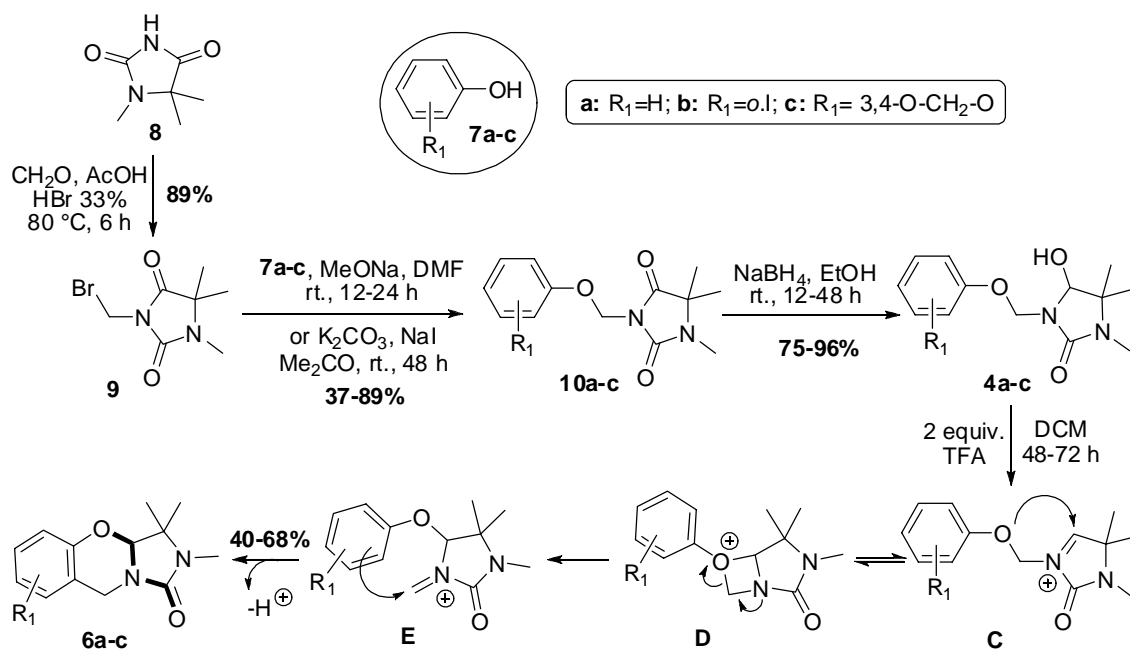
Scheme 2. Scheme leading to the tricyclic targets 6a-c via the effective intramolecular \alpha -oxoalkylation / isomerization / \pi -cationic cyclization cascade.
