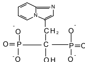
(1-Hydroxy-2-imidazo-(1,2-a)-pyridin-3-yl)- ethylidene bisphosphonate, ( YH529 )
