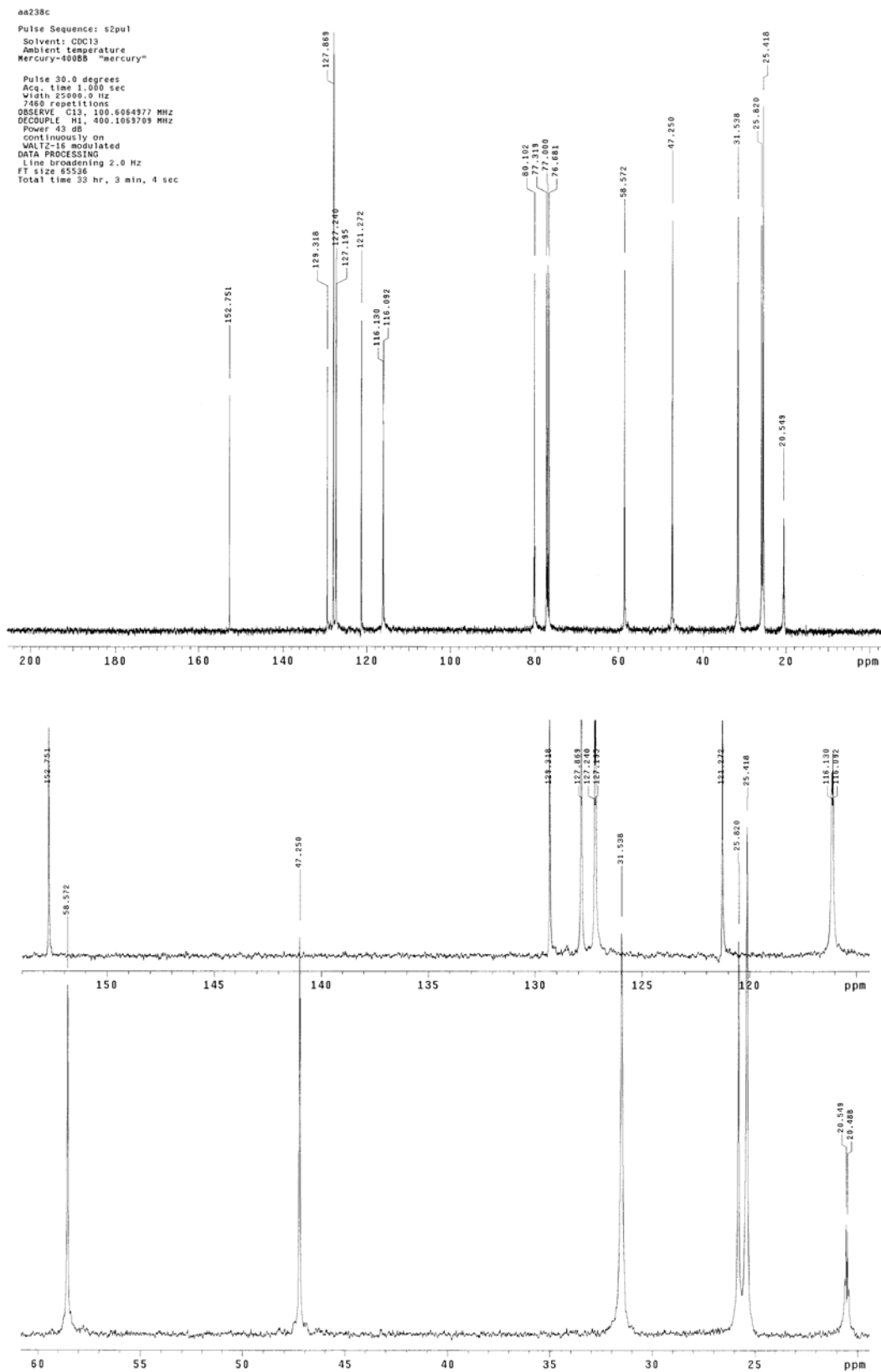
Figure 12. 13 C NMR spectrum of compound 5a.
