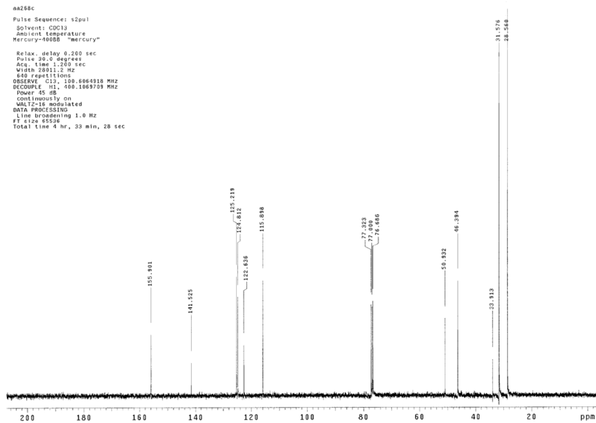
Figure 6. ^{13}\text{C} NMR spectrum of compound 4c.
