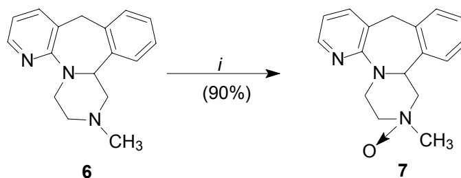
Scheme 2. i. \text{CH}_3\text{CO-OOH} , \text{CH}_2\text{Cl}_2 , rt.
