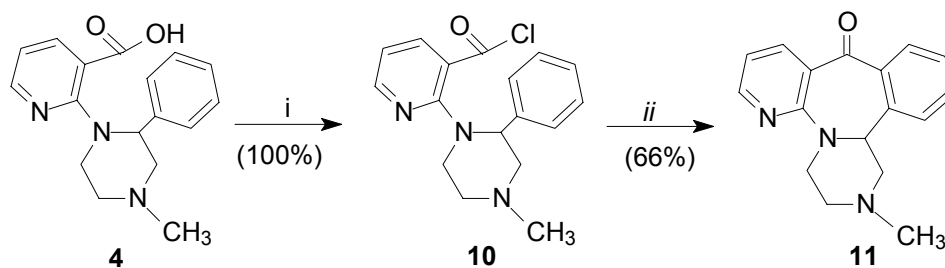
Scheme 4. i. \text{SOCl}_2 , TEA, \text{CH}_2\text{Cl}_2 , reflux; ii. \text{AlCl}_3 , \text{CH}_2\text{Cl}_2 , rt.
