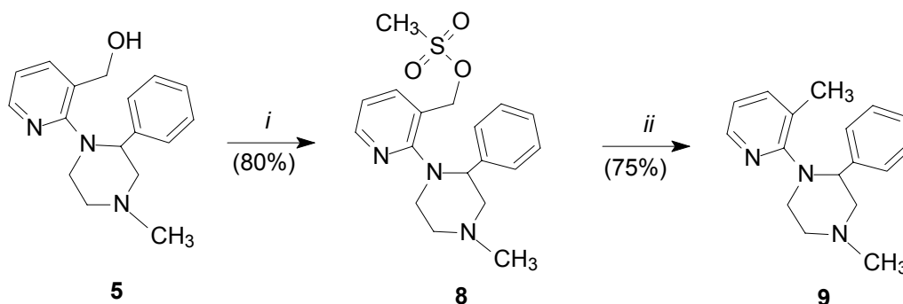
Scheme 3. i. \text{CH}_3\text{SO}_2\text{Cl} , \text{CH}_2\text{Cl}_2 , reflux; ii. \text{LiAlH}_4 , THF, reflux.
