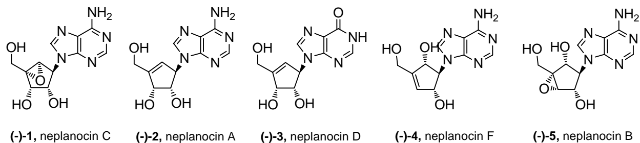
Figure 1. Chemical structures of the neplanocin family of naturally occurring carbanucleosides.
